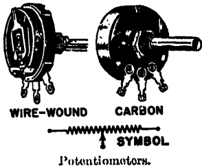
Potentiometers.
